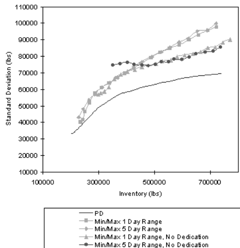
Figure 3: Inventory vs. Inventory Standard Deviation
