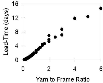
Figure 8: Yarn to Frame Ratio vs. Order Lead-Time
