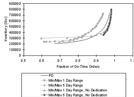
Figure 2: Percentage of On-Time Orders vs. Inventory
