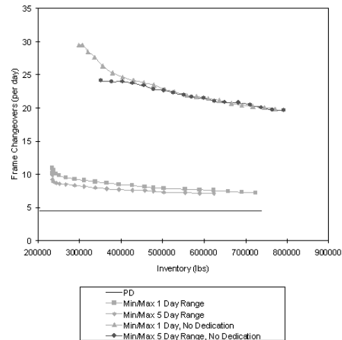
Figure 4: Inventory vs. Frame Changeovers
